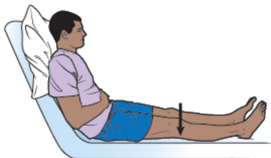
Figure 3. Quadricep sets
