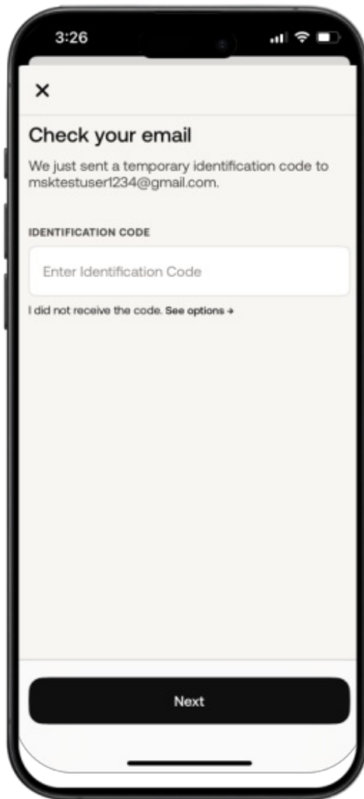
Figure 4. Verification screen
