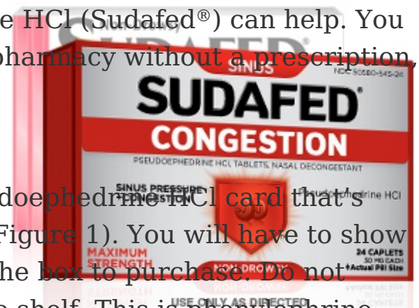
Figure 1. Pseudoephedrine HCl (Sudafed)
