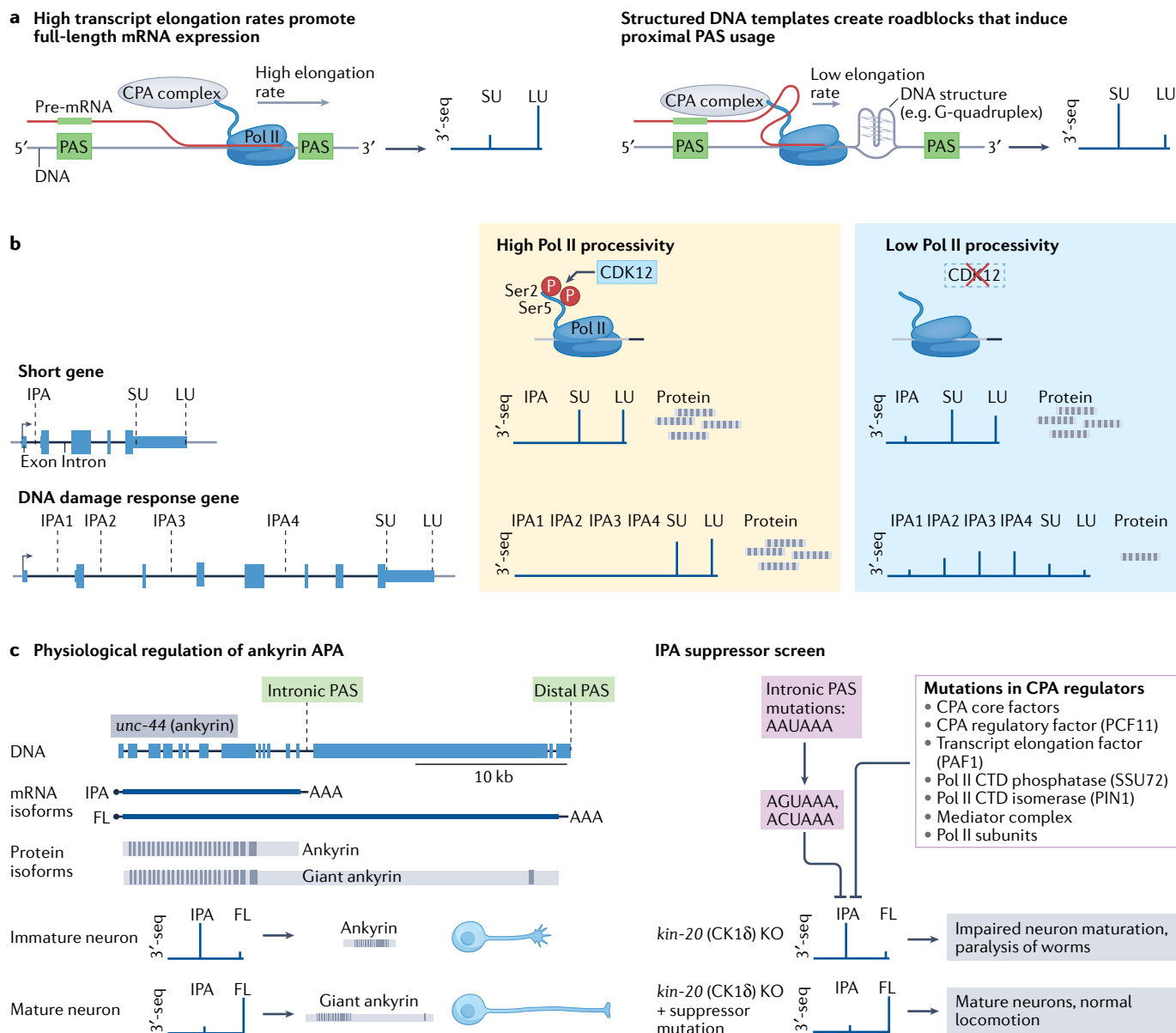
Fig. 3 | Co-transcriptional regulators of alternative polyadenylation.
