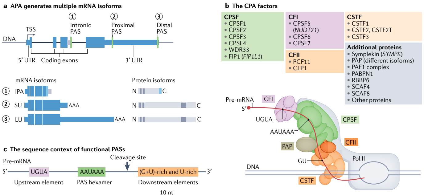
Fig. 1 | Cleavage and polyadenylation of mRNA isoforms at their 3' ends. a | Alternative cleavage and polyadenylation (APA) generates mRNA isoforms that differ in their 3' untranslated regions (UTRs). mRNA processing at intronic polyadenylation (IPA) sites generates mRNA isoforms (IPA isoforms) that encode proteins with alternative C-termini (light blue part of protein). mRNA processing at proximal or distal polyadenylation sites (PASs) in terminal exons generates mRNA isoforms with short 3' UTRs (SU) or long 3' UTRs (LU) that encode proteins with the same amino acid sequence. The grey boxes in the protein symbols represent protein domains. Introns are not drawn to scale. b | During transcription by RNA polymerase II (Pol II), the cleavage and polyadenylation (CPA) machinery binds the PAS hexamer motif AAUAAA and surrounding sequence elements in the nascent RNAs. Shown are CPA factors bound to the pre-mRNA (or nascent RNA) and to the C-terminal domain of Pol II while it is transcribing DNA. The different CPA protein
