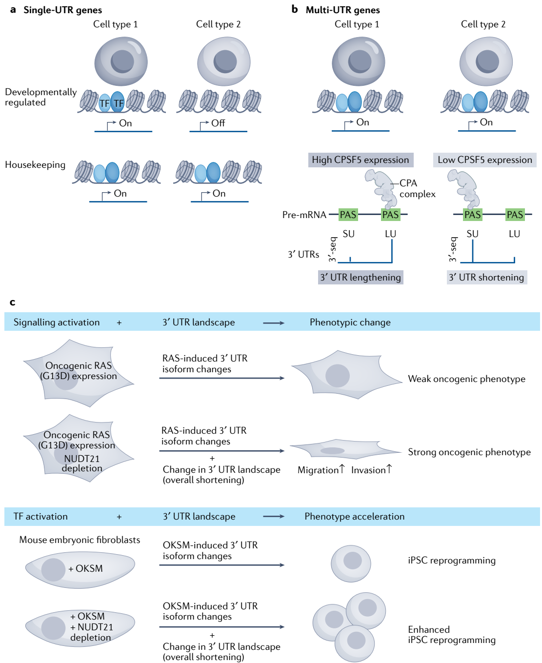
Fig. 5 | Cell-type-specific regulation of single-UTR and multi-UTR genes is accomplished by different regulatory modes. a | Chromatin accessibility and transcription factor (TF) binding determine cell-type-specific transcription of genes whose mRNAs contain a single 3' untranslated region (UTR) isoform (single-UTR genes). b | Multi-UTR genes are widely transcribed (like single-UTR housekeeping genes) yet change their 3' UTR isoforms in a cell-type-specific manner. The cell-type-specific 3' UTR landscape is determined largely by cell-type-specific expression of regulators of alternative cleavage and polyadenylation, such as cleavage and polyadenylation specificity factor subunit 5 (CPSF5; encoded by NUDT21 ). c | Cooperativity between a cell-type-specific 3' UTR landscape and activation of signalling pathways or transcription factors determines phenotypic outcomes. 3'-seq, 3'-end sequencing; CPA, cleavage and polyadenylation; iPSC, induced pluripotent stem cell; LU, long 3' UTR; OKSM, OCT4, KLF4, SOX2 and MYC; PAS, polyadenylation site; SU, short 3' UTR.
