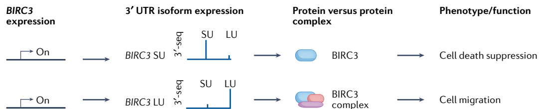
Fig. 6 | Examples of functions of alternative 3' UTRs. a | 3' untranslated region (UTR)-dependent increase in protein synthesis. Cytoplasmic polyadenylation element-binding protein 2 (CPEB2) binds to the long 3' UTR (LU) isoform of the uncoupling protein 1 gene ( Ucp1 ), which increases translation efficiency and protein abundance of UCP1. b | 3' UTR-dependent mRNA localization facilitates synthesis of proteins at their final destination. Shown is a general example of local protein synthesis at the synapse of neurons. c | 3' UTR-dependent local translation in condensates enables protein complex formation. (A+U)-rich elements represent the binding sites for the RNA-binding protein TIS11B. mRNAs that contain these elements in their 3' UTRs localize to TIS granules, whereas lack of these elements results in localization to the endoplasmic reticulum (ER) or to the cytoplasm. Local protein synthesis in TIS granules allows the formation of protein complexes that cannot be established upon translation outside this cytoplasmic condensate. Shown is the compartment-dependent assembly of the complex between CD47 and SET, which traffics CD47 more efficiently to the plasma membrane, where it represses phagocytosis. d | 3' UTR-dependent protein complex assembly determines protein function. A change in 3' UTR isoform expression of the gene encoding the ubiquitin ligase BIRC3 leads to assembly of a protein complex, which changes BIRC3 function in human cells. 3'-seq, 3'-end sequencing; LU, long 3' untranslated region; SU, short 3' untranslated region.
