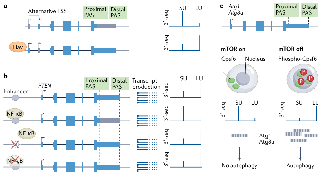
Fig. 4 | Gene-specific regulation of alternative 3' UTR isoforms. a | Differential binding of factors at alternative transcription start sites can mediate gene-specific regulation of alternative polyadenylation site (PAS) use. In fly neurons, the RNA-binding protein embryonic lethal abnormal visual system (Elav) binds to specific promoters and transcription start sites (TSS) and thus controls the expression of mRNAs with longer 3' untranslated regions (UTRs). b | Transcription factors that bind to specific enhancers regulate APA in a gene-specific manner. Signalling-induced activation of nuclear factor- \kappa B (NF- \kappa B) induces its binding to a specific enhancer of the phosphatase and tensin homologue gene ( PTEN ) in human cell lines. NF- \kappa B activation does not change the production or stability of the PTEN mRNA, but induces a change in 3' UTR isoform expression. Deletion of the enhancer or silencing of NF- \kappa B impairs this signalling-induced APA change. c | Signalling-induced phosphorylation of cleavage and polyadenylation specificity factor subunit 6 (Cpsf6) increases its activity and promotes autophagy. In flies, inactivation of the mTOR pathway allows expression of two kinases (not shown) that phosphorylate Cpsf6 in the cytoplasm, thereby promoting its translocation to the nucleus and RNA-binding activity. Cpsf6 changes the APA pattern of two master regulators of autophagy, the autophagy-related protein 1 gene ( Atg1 ) and Atg8a . Increased expression of their long 3' UTR (LU) isoforms supports high-level protein expression, thereby inducing autophagy upon mTOR inhibition to allow intracellular nutrient uptake. 3'-seq, 3'-end sequencing; SU, short 3' UTR.
