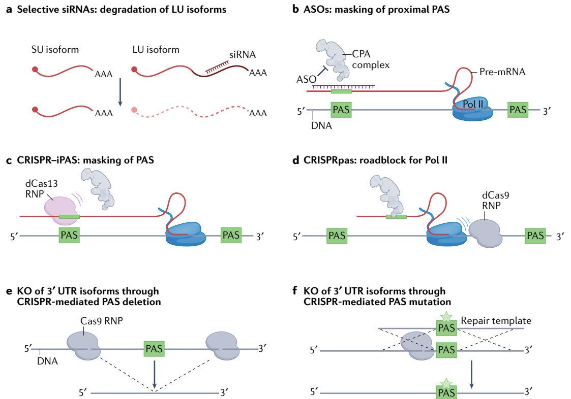
Fig. 7 | Manipulation of alternative 3' UTR expression. a | Small hairpin RNAs or small interfering RNAs (siRNAs) targeting the extended part of 3' untranslated region (UTR) isoforms exclusively downregulate the expression of long 3' UTR (LU) isoforms. b | Antisense oligonucleotides (ASOs) that are complementary to a specific proximal polyadenylation site (PAS) prevent binding of the cleavage and polyadenylation (CPA) machinery and exclusively downregulate expression of short 3' UTR (SU) isoforms. c | CRISPR-iPAS. An enzymatically dead Cas13 (dCas13) is targeted by a guide RNA (dCas13 RNP) to a region slightly upstream of a PAS of interest, where it prevents CPA factors from recognizing the PAS. d | CRISPRpas. An enzymatically dead Cas9 (dCas9) is targeted by a guide RNA to a region downstream of a PAS of interest, where it acts as a roadblock for RNA polymerase II (Pol II) elongation, thereby increasing CPA at the PAS. e | Permanent removal of a specific PAS or entire 3' UTR isoforms using a pair of Cas9 RNPs to delete the region of interest. f | PAS mutagenesis through homologous recombination can be achieved by CRISPR-Cas9-mediated DNA cleavage in the presence of a homologous repair template that contains the mutation. Cas RNP, Cas protein-guide RNA complex; KO, knockout.
