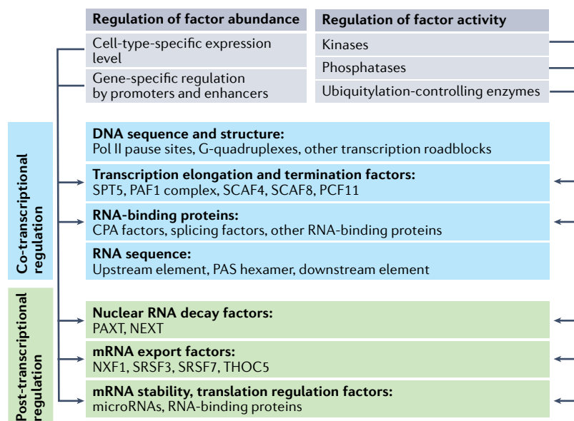
Fig. 2 | Overview of regulation of alternative polyadenylation by co-transcriptional and post-transcriptional mechanisms. Alternative cleavage and polyadenylation (APA) is regulated both co-transcriptionally and post-transcriptionally. Cis-regulatory elements in the RNA and the DNA are necessary but not sufficient for cleavage and polyadenylation (CPA). As CPA occurs while RNA polymerase II (Pol II) transcribes a gene, Pol II elongation dynamics regulate APA. A selection of APA-regulating factors is given. Pol II termination factors show extensive crosstalk with RNA-binding proteins such as splicing factors and CPA factors that recognize RNA sequence elements and control where and when a pre-mRNA is cleaved and polyadenylated. Following processing of 3' untranslated region isoforms, the expression level of individual APA isoforms is further regulated by post-transcriptional processes. Both the abundance and the activity of factors that control APA can be regulated co-transcriptionally and post-transcriptionally, often in a cell-type-specific and condition-specific manner, thereby allowing dynamic regulation of APA at individual genes. NEXT, nuclear exosome targeting (a trimeric protein complex); NXF1, nuclear RNA export factor 1; PAF1, RNA polymerase II-associated factor 1; PAXT, poly(A) tail exosome targeting (a trimeric protein complex); SCAF4, serine and arginine-related C-terminal domain-associated factor 4; SPT5, suppressor of Ty 5; SRSF, serine and arginine-rich splicing factor 3; THOC5, THO complex 5.
